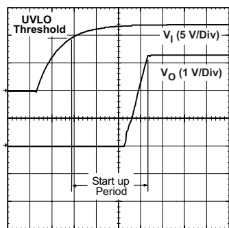
Figure 18. PTH12020W Startup
