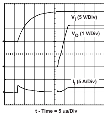
Figure 11. Power-Up Waveforms
