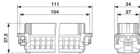
Female insert
