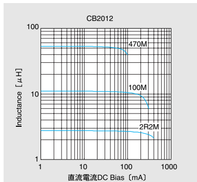
直流量重畳特性例 DC Bias characteristics (Measured by HP4285A+42841A)
