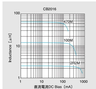
直流量重畳特性例 DC Bias characteristics (Measured by HP4285A+42841A)
