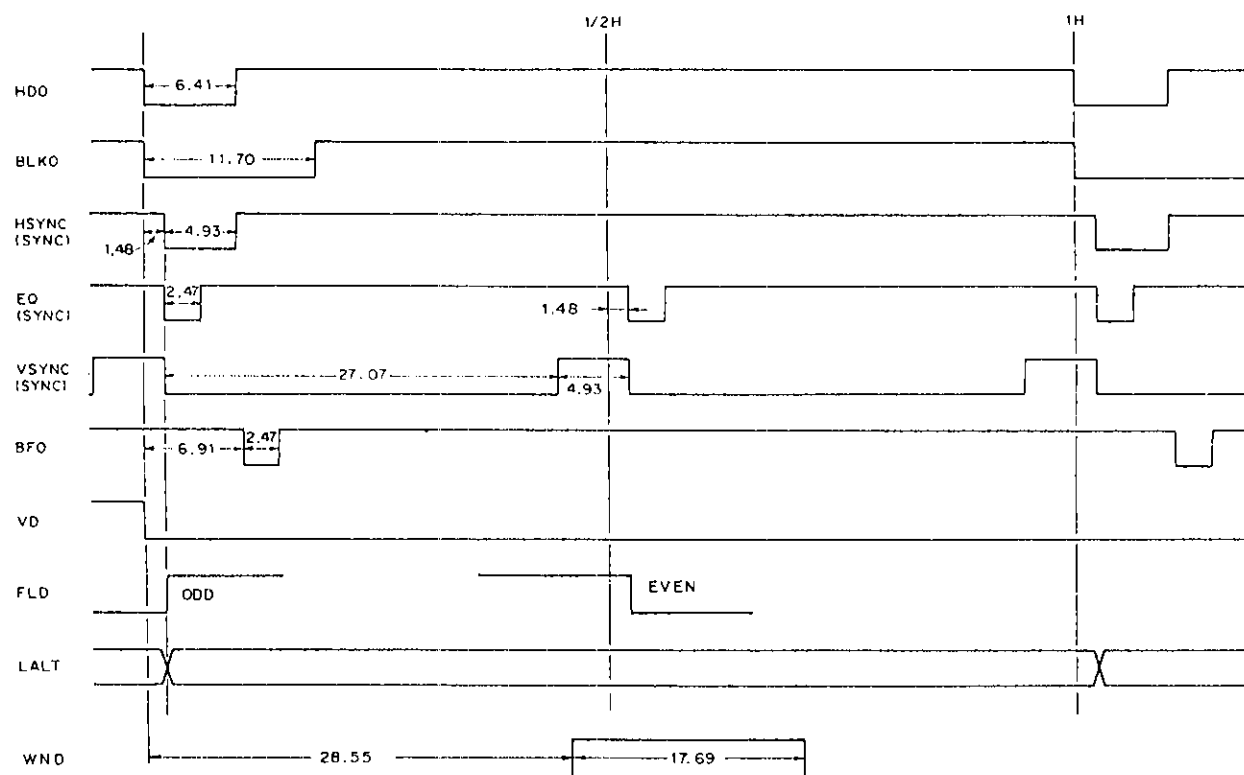
Timing Chart H (PAL)
