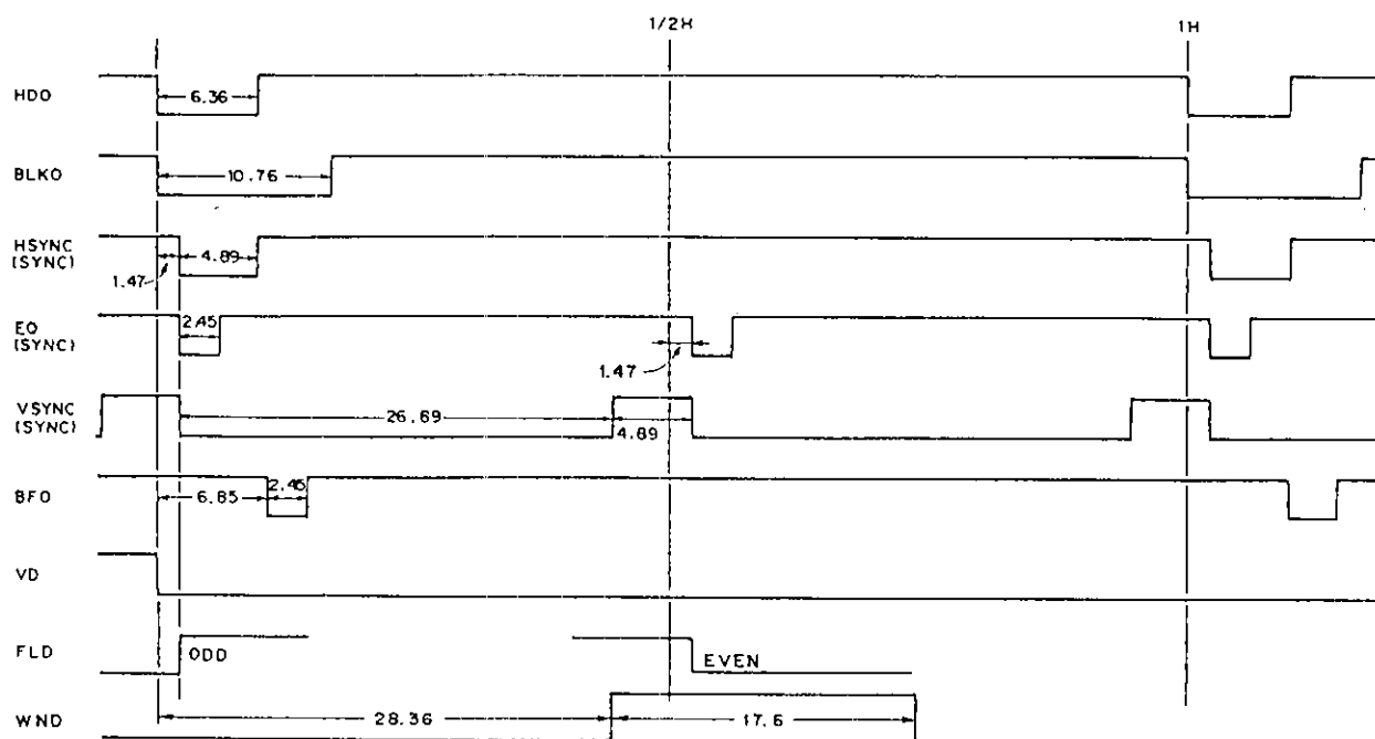
Timing Chart H (NTSC)
