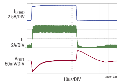
Load Transient Response, Pulse Skip Mode
