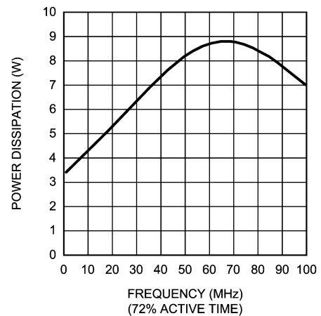
FIGURE 6. Power Dissipation vs Frequency
