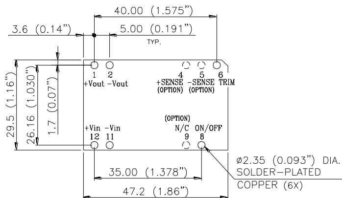
BOTTOM VIEW
