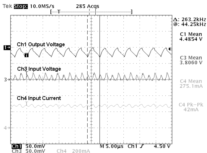
Output Ripple on 4.5V Output at 262kHz
