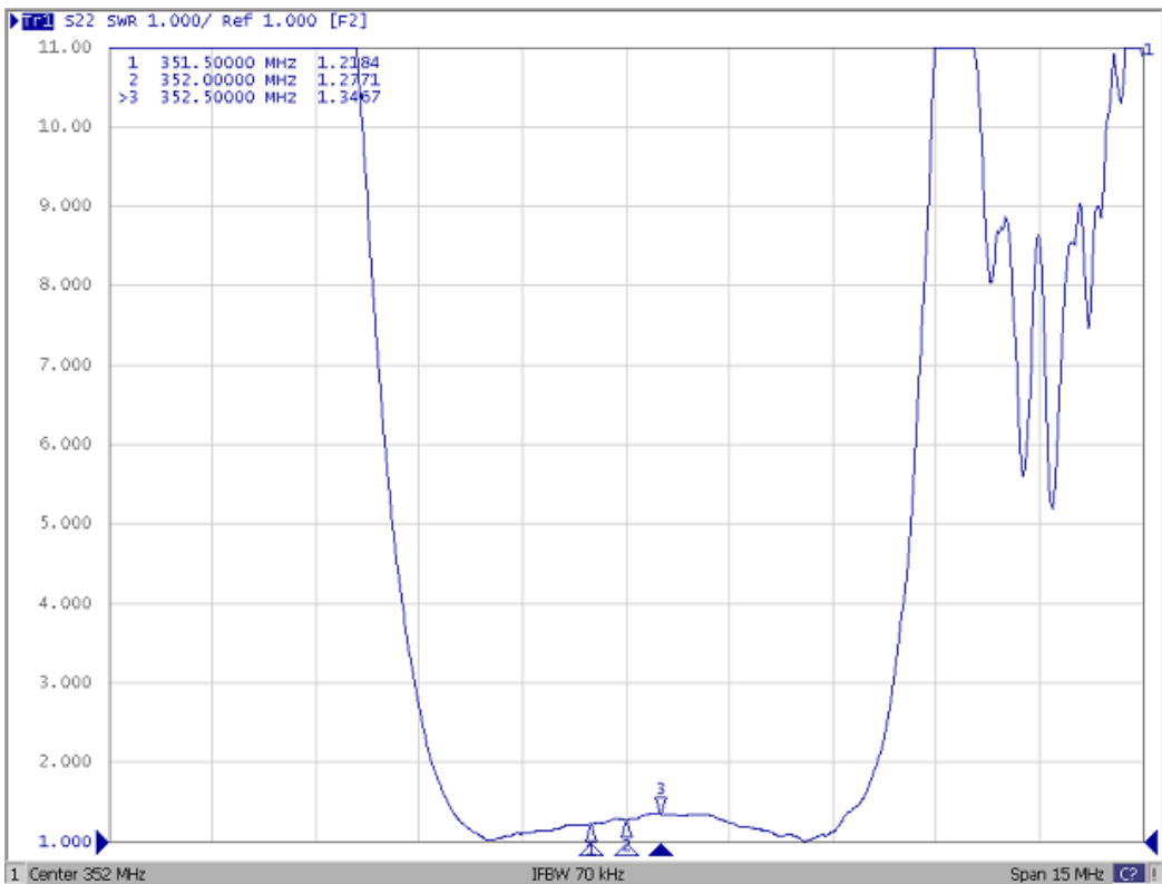
S22
