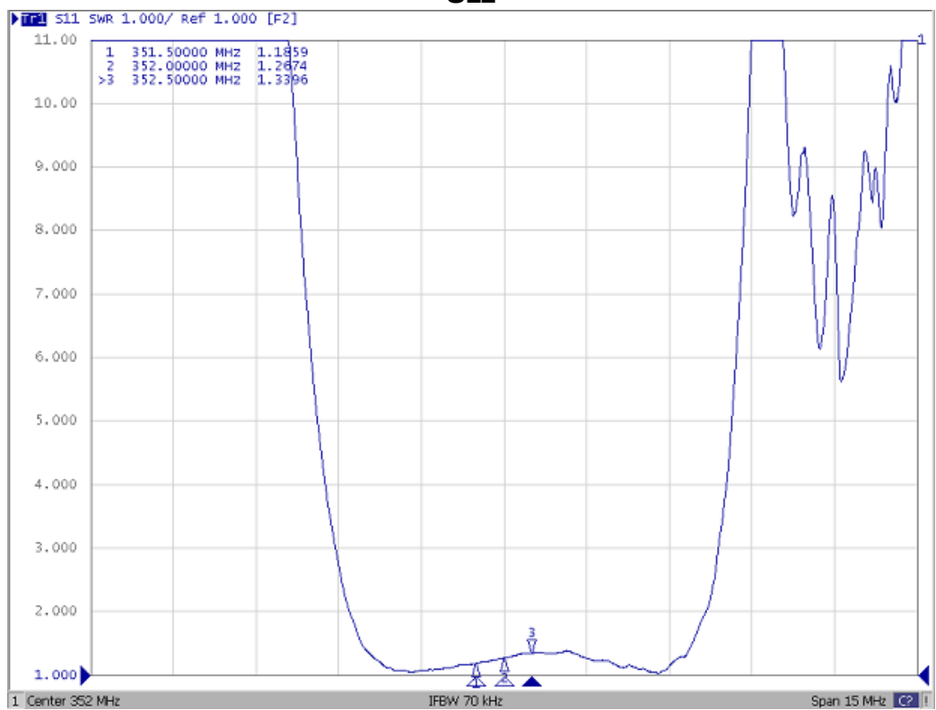
S11
