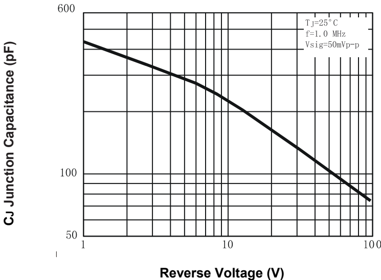
Fig.5-Typical junction capacitance
