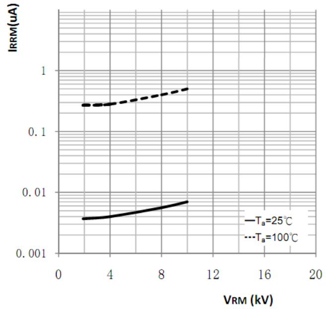
Reverse Characteristics
