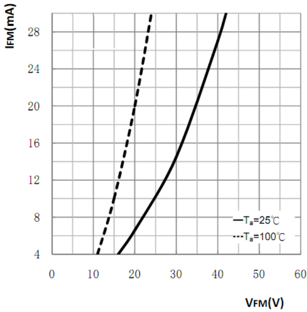
Forward Characteristics
