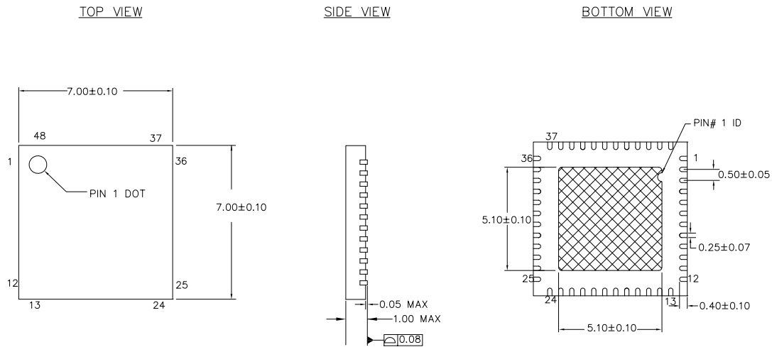
Figure 24. 48-pin QFN ( 7 \times 7 \times 1.0 mm) LT48A 5.1 \times 5.1 E-Pad (Sawn) Package Outline, 001-13191
