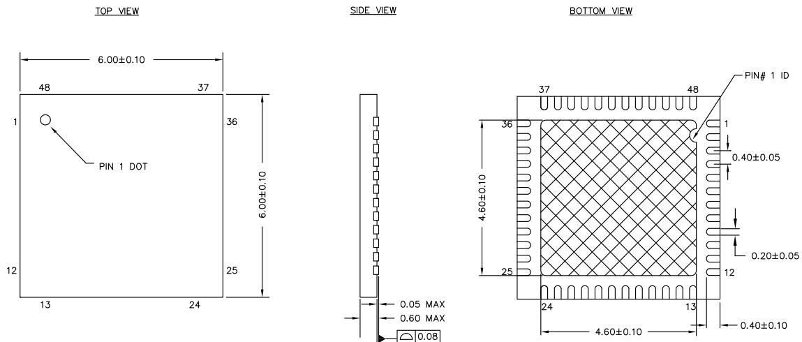
Figure 25. 48-pin QFN ( 6 \times 6 \times 0.6 mm) LQ48A 4.6 \times 4.6 E-Pad (Sawn) Package Outline, 001-57280
