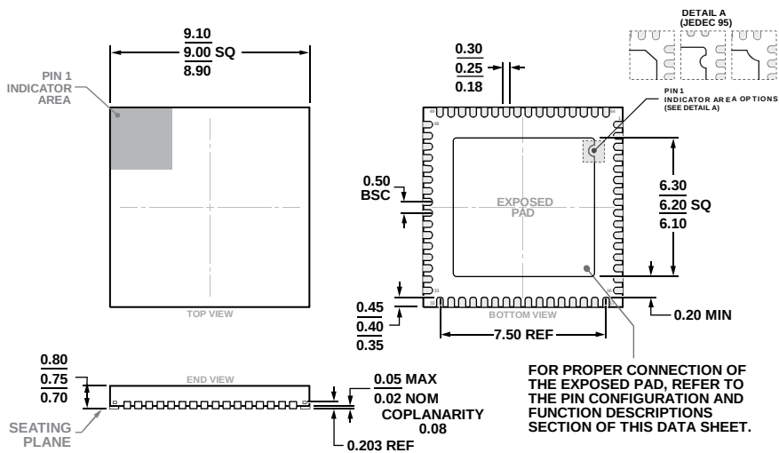
Figure 30. 64-Lead Lead Frame Chip Scale Package [LFCSP] 9 mm × 9 mm Body and 0.75 mm Package Height (CP-64-17)
