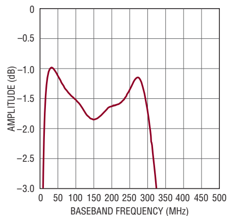
Figure 17. Baseband Frequency Response
