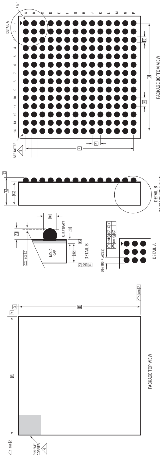
BGA Package 196-Lead (15mm × 15mm × 2.82mm) (Reference LTC DWG# 05-08-1907 Rev D)
