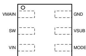
图 6-1. DSE Package 6-Pin WSON Top View
