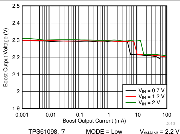
图 7-28. Boost Load Regulation (Low Power Mode)
