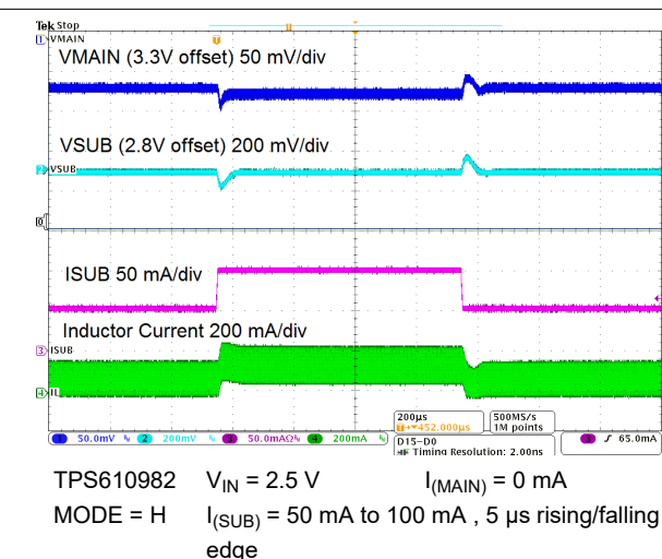
图 9-35. LDO Load Transient Response
