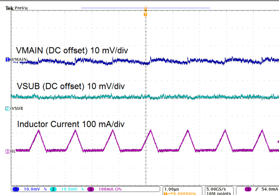
图 9-5. Switching Waveforms
