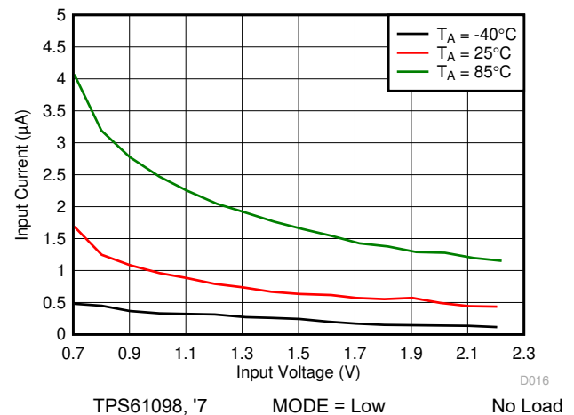
图 7-42. Input Current vs Input Voltage (Low Power Mode)
