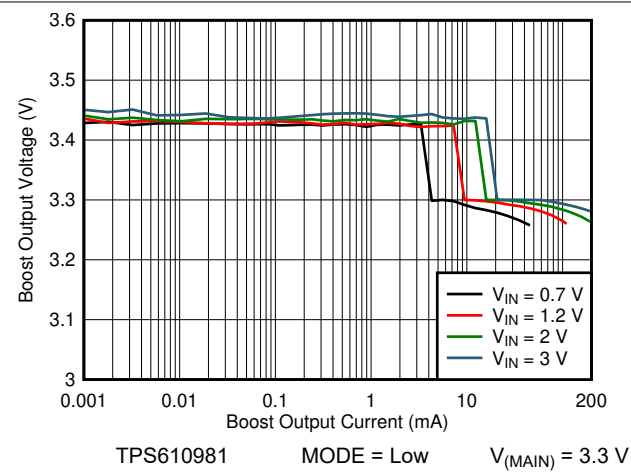
图 7-30. Boost Load Regulation (Low Power Mode)
