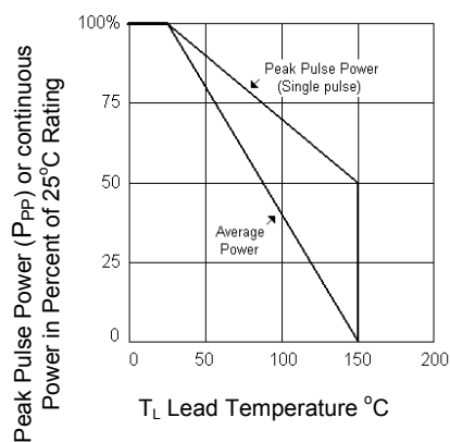
FIGURE 3 - Derating Curve
