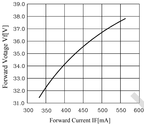
Forward Votage Vs. Forward Current
