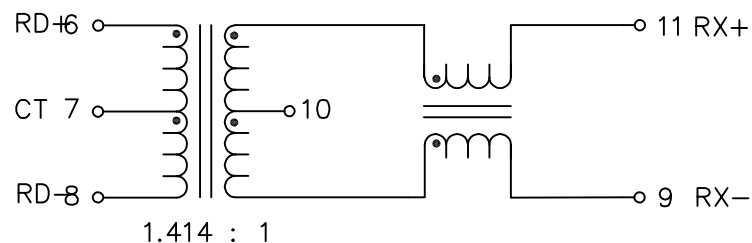
SCHEMATIC
