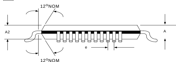
Figure 5 - LQFP-100
