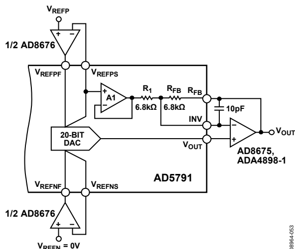
Figure 52. Output Amplifier in Gain of Two Configuration
