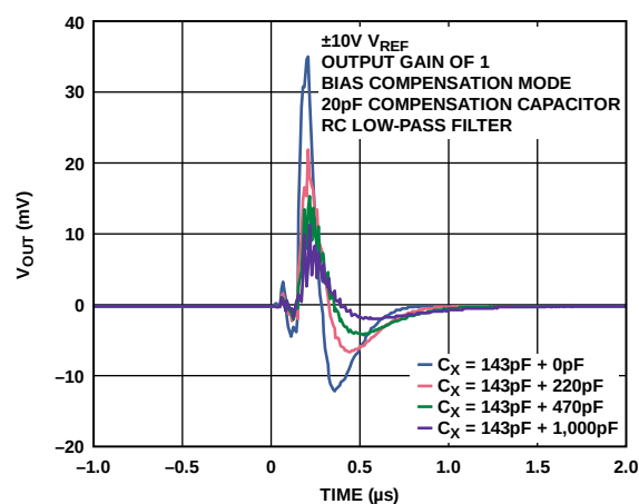
Figure 45. Midscale Peak-to-Peak Glitch for ±10 V_{REF}
