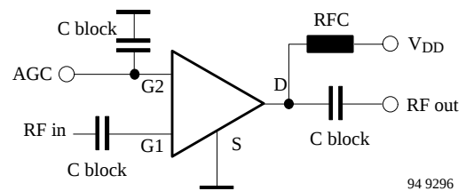
Amplifier 2
