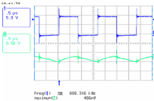
Fig.4. CH1: PWM waveform, CH2, v_{p-p} for V_o
