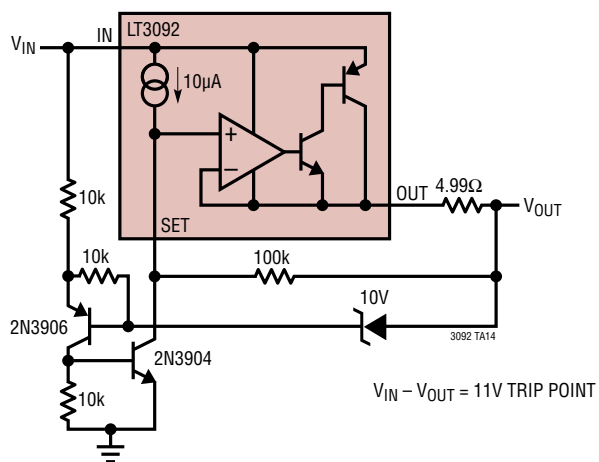
Voltage Clamp
