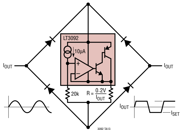
2-Terminal AC Current Limiter
