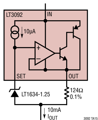
High Accuracy Current Source
