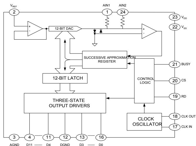
Logic Diagram
