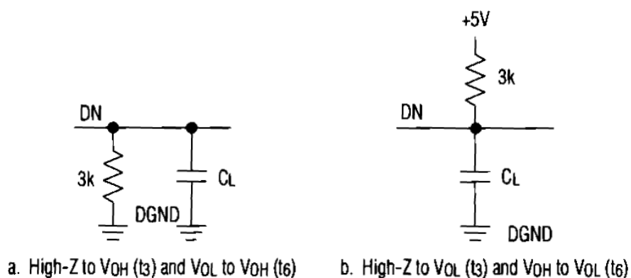
FIGURE 1. LOAD CIRCUITS FOR ACCESS TIME
