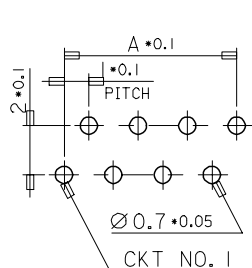
P.C. BOARD LAYOUT (MOUNTING SIDE) (THK. : 1.6t)
