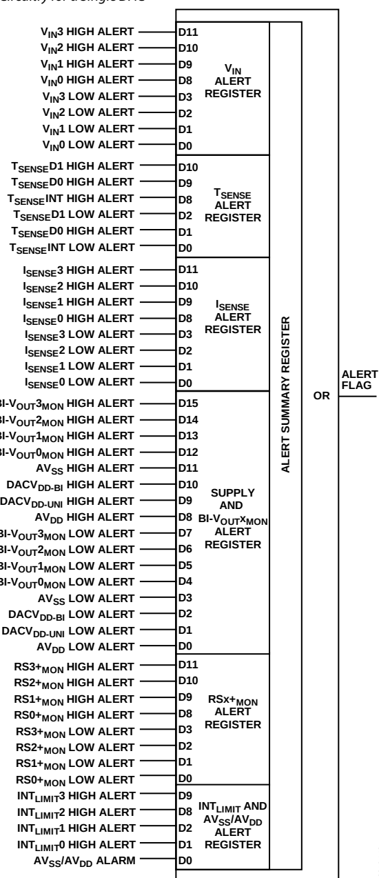
Figure 49. Software Alerts Page
