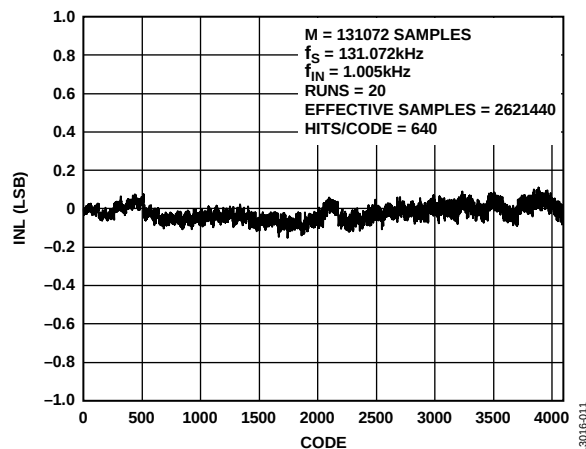
Figure 11. ADC INL Single-Ended, \text{REF}_{\text{ADC}} Range
