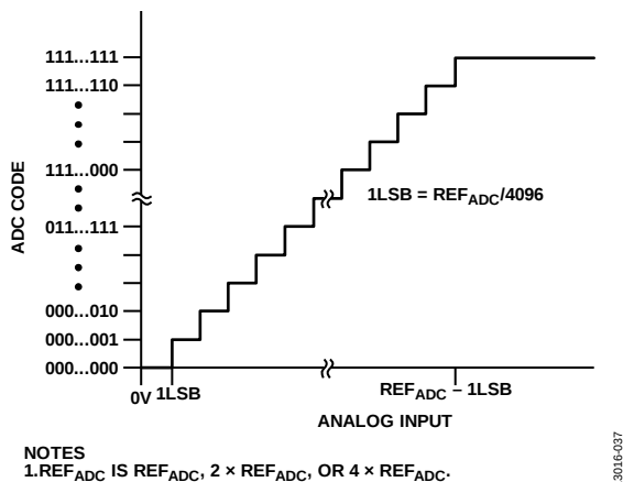
Figure 35. Single-Ended Transfer Characteristics
