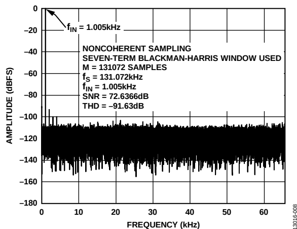
Figure 8. Signal-to-Noise Ratio, Single-Ended Input, 2 \times \text{REF}_{\text{ADC}} Range
