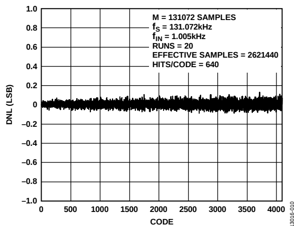
Figure 10. ADC DNL Single-Ended, \text{REF}_{\text{ADC}} Range
