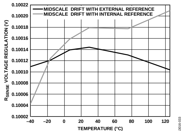
Figure 31. Closed-Loop R_{SENSE} Voltage Regulation vs. Temperature
