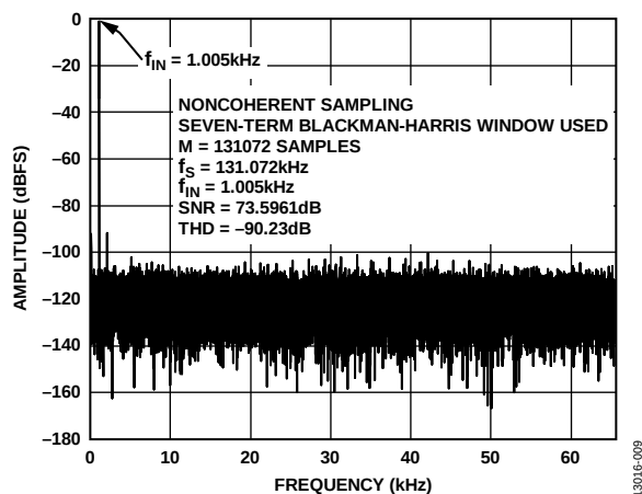
Figure 9. Signal-to-Noise Ratio, Differential Input, \text{REF}_{\text{ADC}} Range
