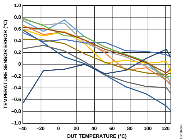
Figure 28. Temperature Sensor Error vs. Device Under Test (DUT) Temperature
