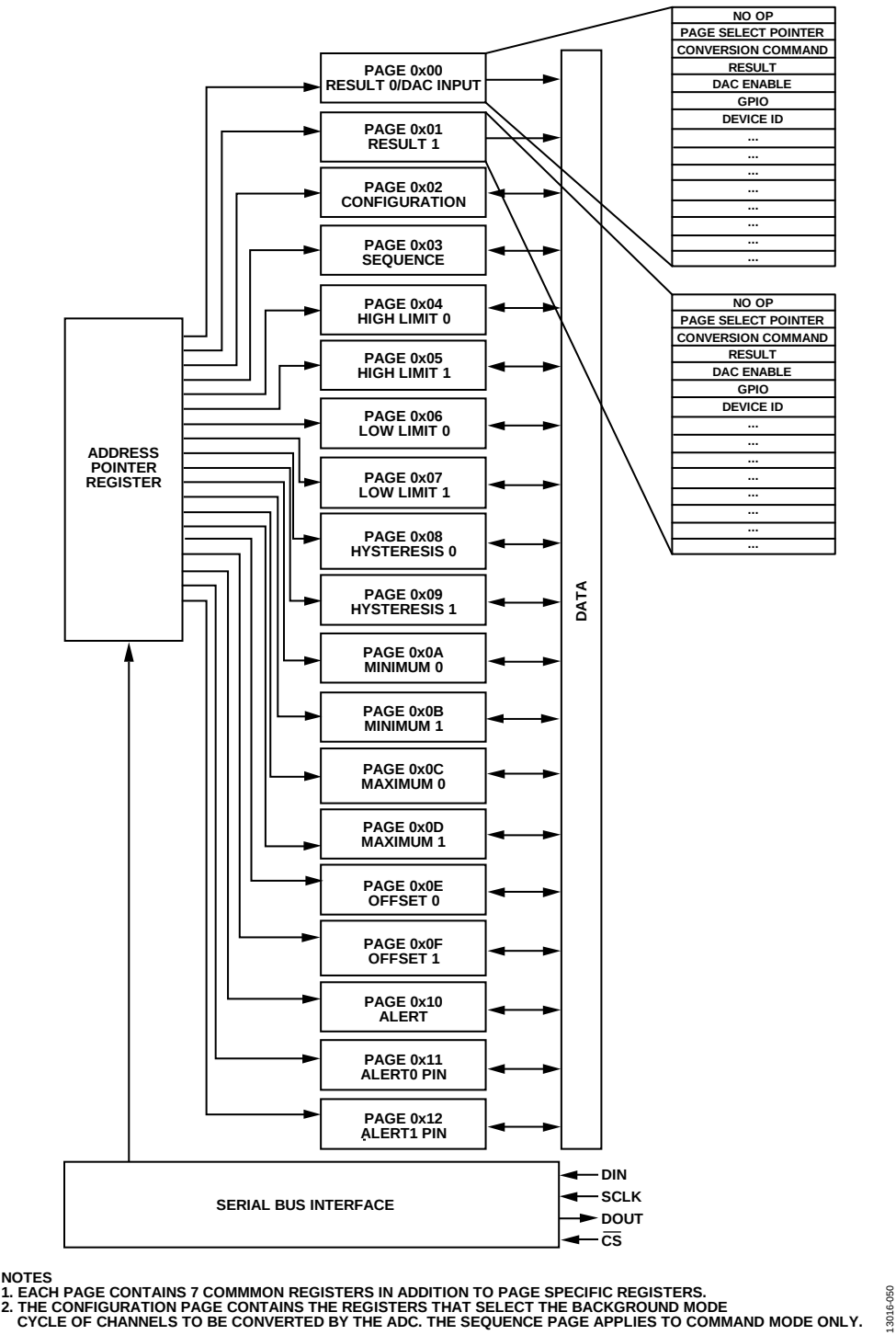
Figure 51. Register Structure
