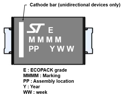
Figure 19. SMA marking
