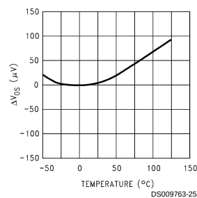
Offset Voltage
