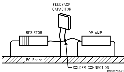
FIGURE 10. Air Wiring
