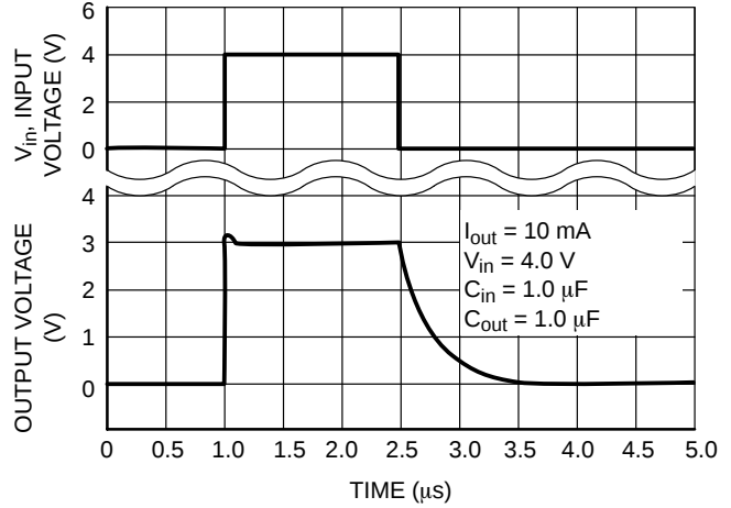
Figure 11. Turn-on Response
