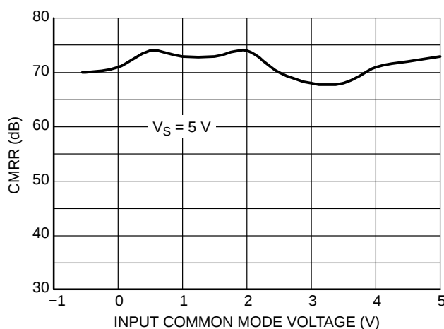
Figure 2. CMRR vs. Input Common Mode Voltage
