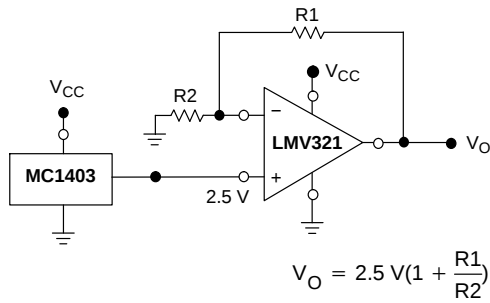
Figure 28. Voltage Reference
