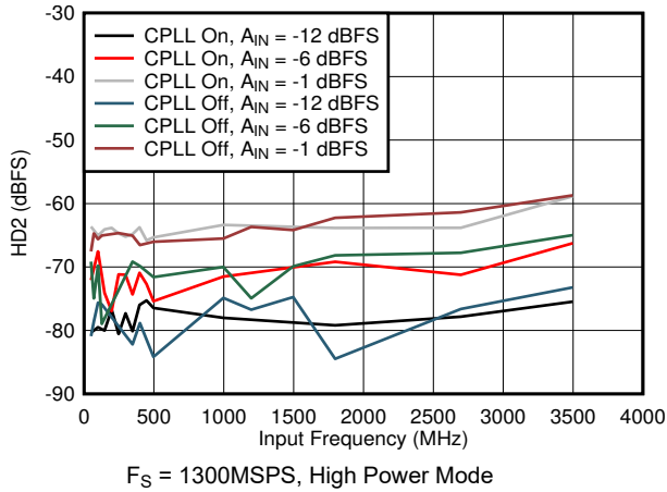
Figure 7-73. HD2 vs Input Frequency, CPLL and Input Amplitude
