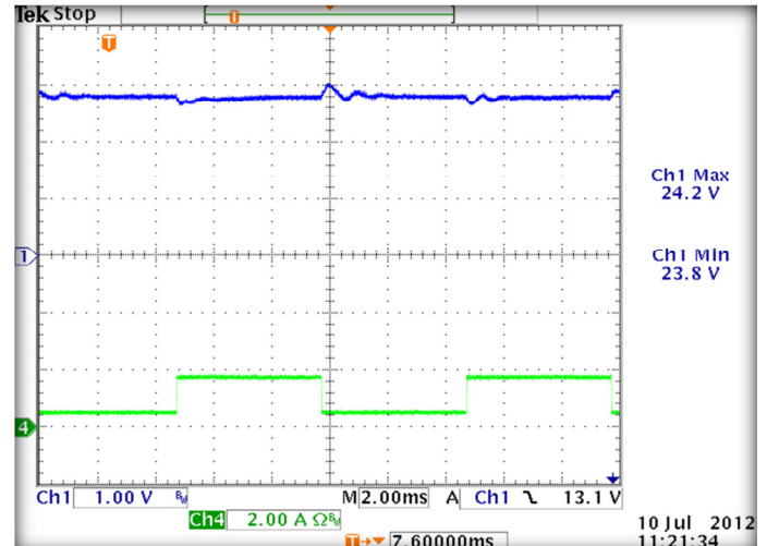
24V OUT, 240VAC, 25% TO 75% LOAD STEP
