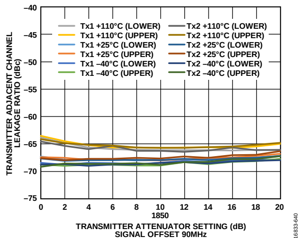
Figure 88. Transmitter Adjacent Channel Leakage Ratio vs. Transmitter Attenuator Setting, Signal Offset = 90 MHz, LO = 1850 MHz, LTE = 20 MHz, PAR = 12 dB, Upper Side and Lower Side
