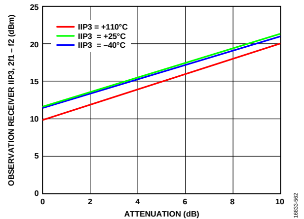
Figure 58. Observation Receiver IIP3, 2f_1 - f_2 vs. Attenuation, LO = 300 MHz, Tone 1 = 345 MHz, Tone 2 = 346 MHz at -24 dBm Plus Attenuation
