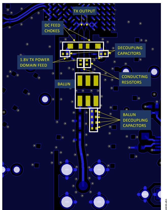
Figure 280. Transmitter DC Chokes and Balun Feed Supply
