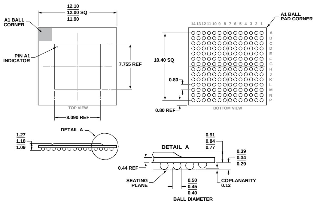
COMPLIANT TO JEDEC STANDARDS MO-275-GGAB-1. Figure 301. 196-Ball Chip Scale Package Ball Grid Array [CSP_BGA] (BC-196-13) Dimensions shown in millimeters
