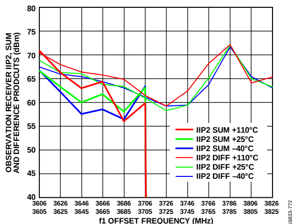
Figure 173. Observation Receiver IIP2, Sum and Difference Products vs. f1 Offset Frequency, Tones Separated by 1 MHz Swept Across Pass Band at -22 dBm Each, LO = 3600 MHz, Attenuation = 0 dB
