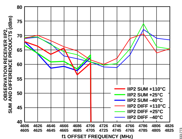
Figure 174. Observation Receiver IIP2, Sum and Difference Products vs. f1 Offset Frequency, Tones Separated by 1 MHz Swept Across Pass Band at -22 dBm Each, LO = 4600 MHz, Attenuation = 0 dB
