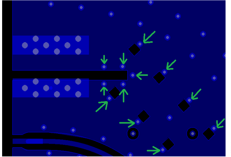
Figure 283. Current Steering Vias Placed Next to Isolation Structures
