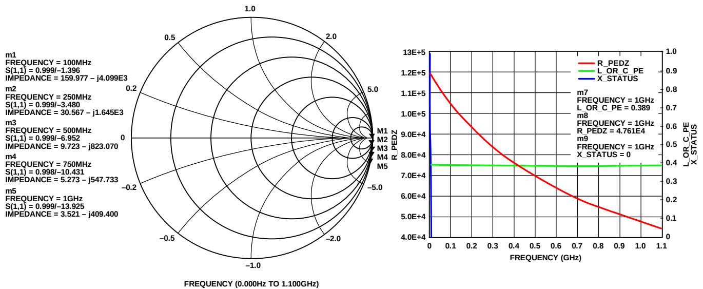
Figure 288. REF_CLK_IN± SEDZ and PEDZ Data, On Average, the Real Part of the Parallel Equivalent Differential Impedance ( R_P ) = ~ 70 k \Omega
