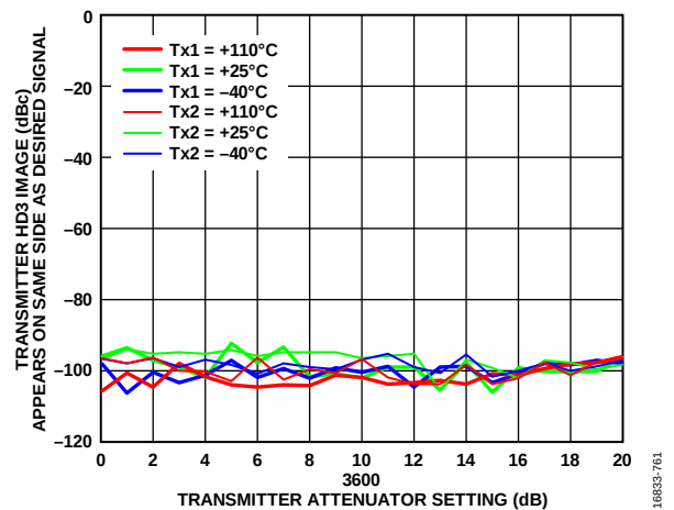
Figure 162. Transmitter HD3 Image Appears on Same Side as Desired Signal vs. Transmitter Attenuator Setting, LO = 3600 MHz, CW = -15 dBFS
