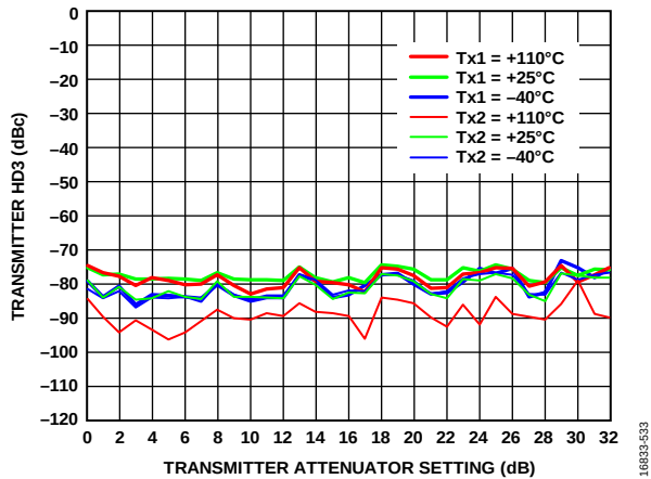
Figure 29. Transmitter HD3 vs. Transmitter Attenuator Setting, LO = 525 MHz, CW = -15 dBFS, Baseband Frequency = 10 MHz
