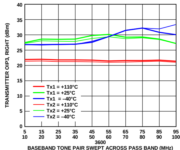
Figure 156. Transmitter OIP3, Right vs. Baseband Tone Pair Swept Across Pass Band, LO = 3600 MHz, Total RMS Power = -12 dBFS
