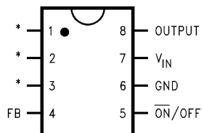
Figure 1. 8-Pin - Top View See Package Number P0008E
