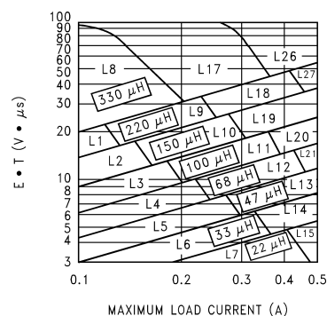
Figure 24. LM2594/LM2594HV-ADJ
