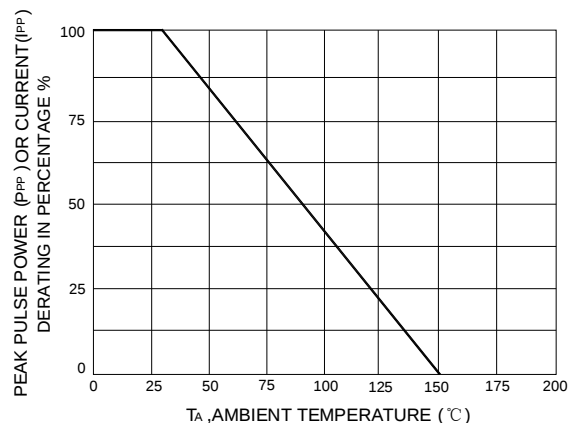
FIG.2- PULSE RATING CURVE
