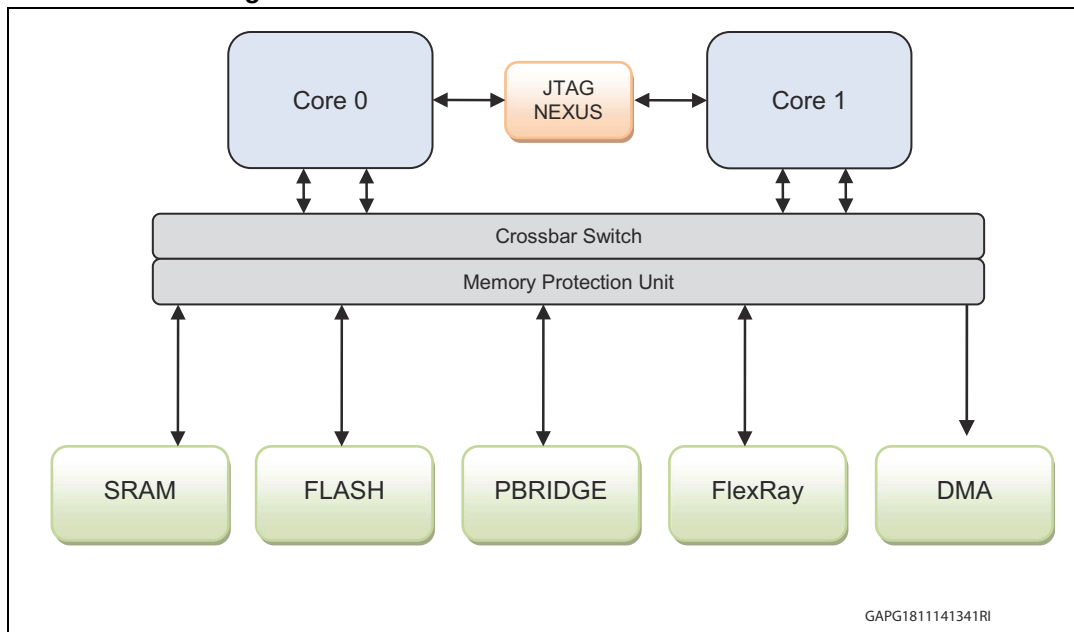
Figure 1. Power Architecture dual-core architecture
