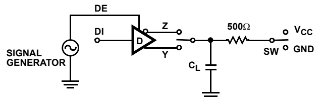
FIGURE 2. DRIVER PROPAGATION DELAY AND DIFFERENTIAL TRANSITION TIMES
