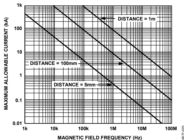
Figure 28. Maximum Allowable Current for Various Current-to- ADuM5401/ADuM5402/ADuM5403/ADuM5404 Spacings
