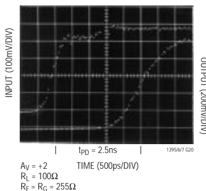
Propagation Delay
