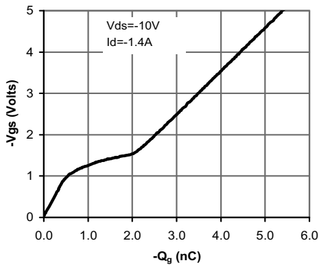
Figure 7: Gate-Charge Characteristics
