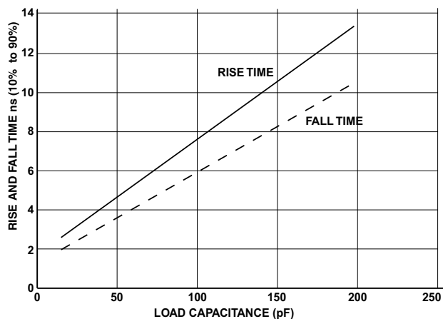
Figure 46. Typical Rise and Fall Times (10% to 90%) vs. Load Capacitance for Driver A at V_{\text{DDEXT}} = 2.7 \text{ V (Min)}
