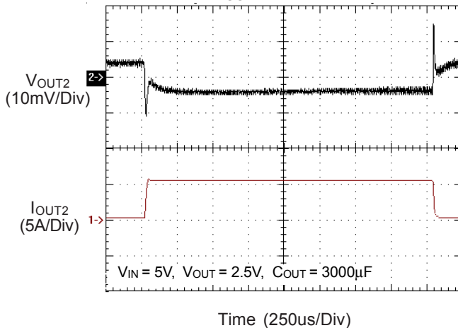
V OUT2 Transient
