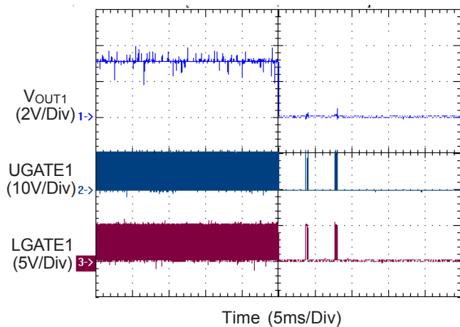
V OUT1 Short
