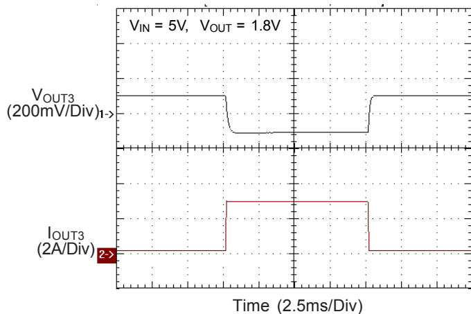
V OUT3 Transient
