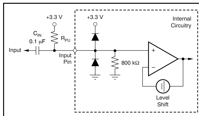
Figure 46. AC-Bias Input Mode Circuit Configuration
