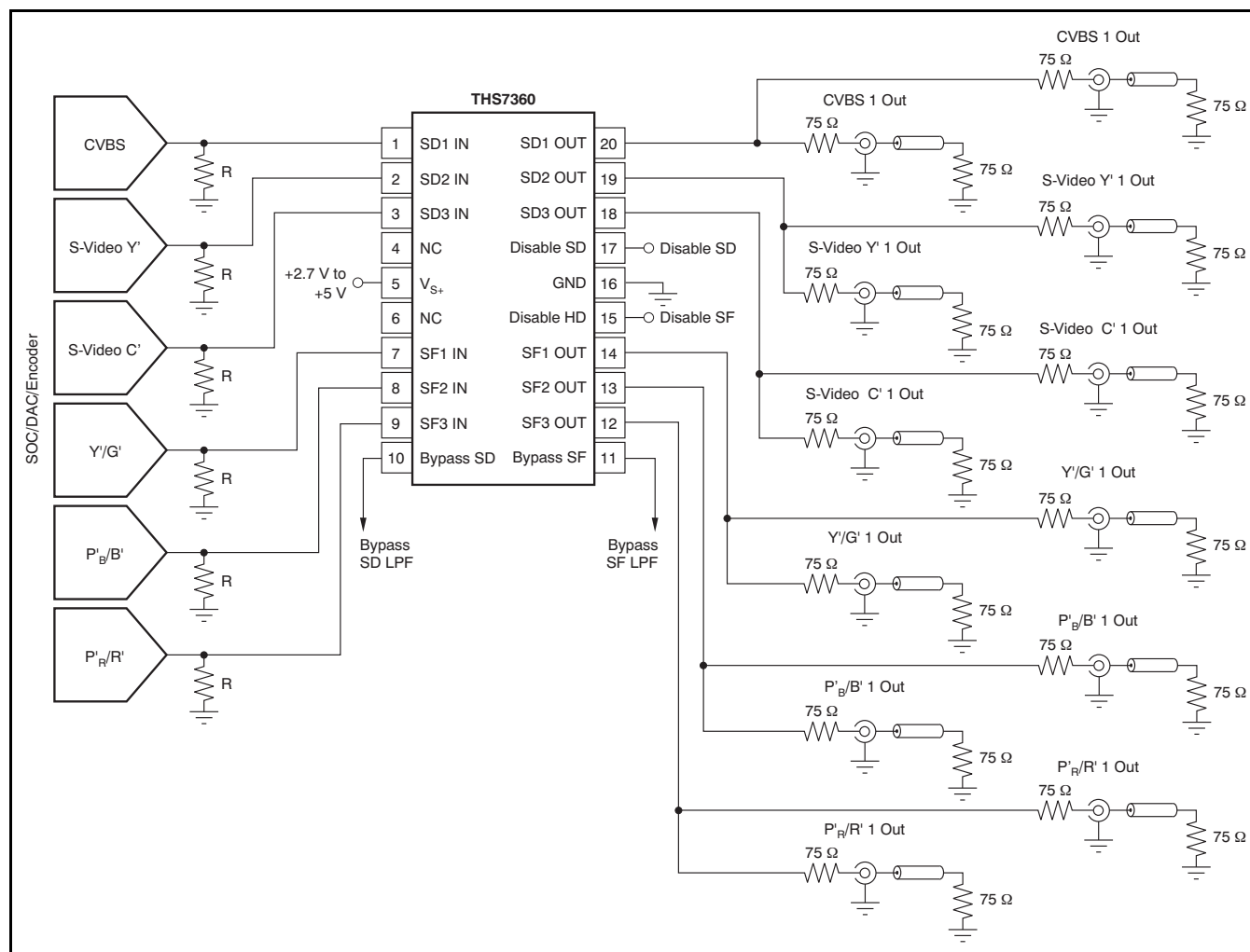
Figure 47. Typical Six-Channel System with DC-Coupled Line Driving and Two Outputs Per Channel
