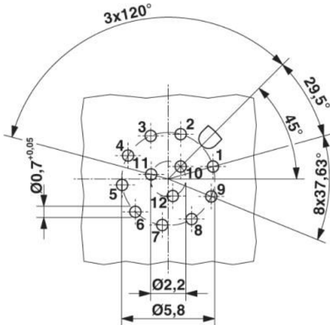
Drilling diagram
