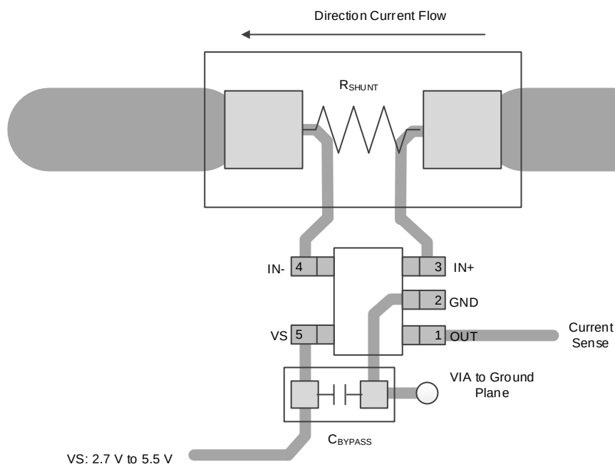
Figure 45. Recommended Layout
