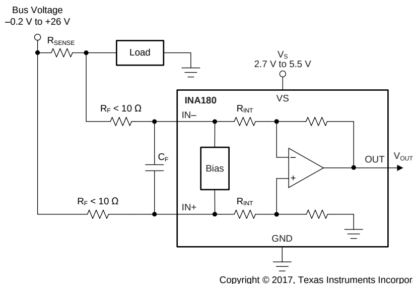
Figure 40. Filter at Input Pins
