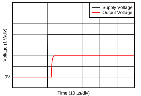
Figure 31. Start-Up Response
