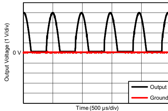
Figure 42. Output Response
