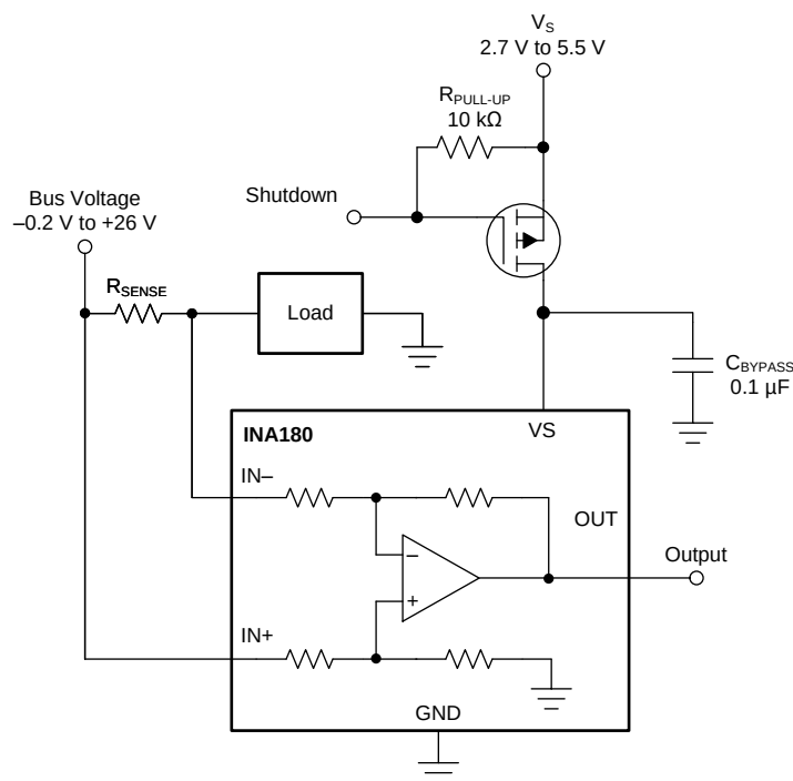
Figure 38. Basic Circuit to Shut Down the INx180
