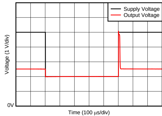
Figure 32. Brownout Recovery
