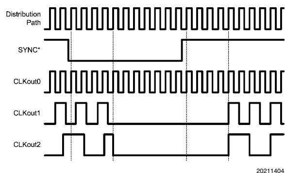
FIGURE 1. SYNC* Timing Diagram
