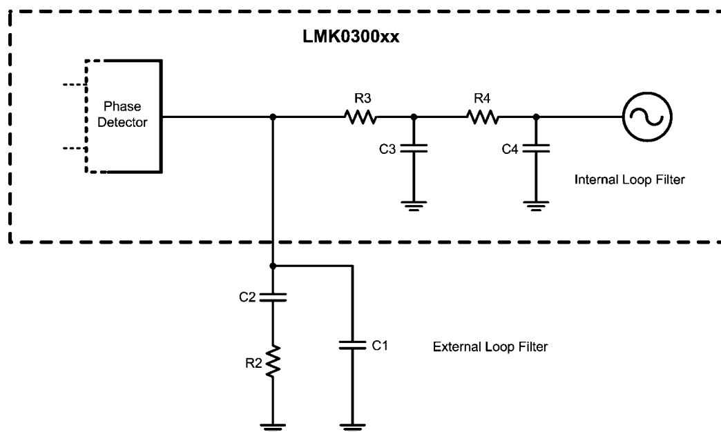
FIGURE 4. Loop Filter
