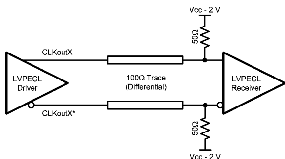
FIGURE 7. Differential LVPECL Operation, DC Coupling
