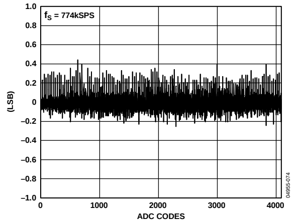
图21. f_s = 774 kSPS时典型DNL误差
