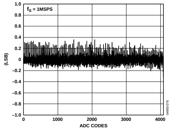
图22. f_s = 1 MSPS时典型DNL误差
