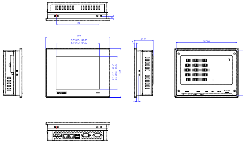
Panel Cut-out Dimensions: 189.1 x 142.1 mm (7.44" x 5.59")
