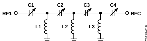
Figure 16. HPF Simplified Schematic
