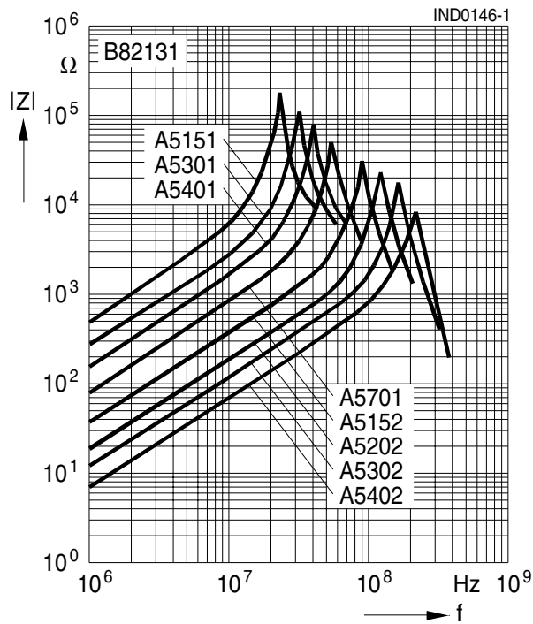
B82131A5***M000
