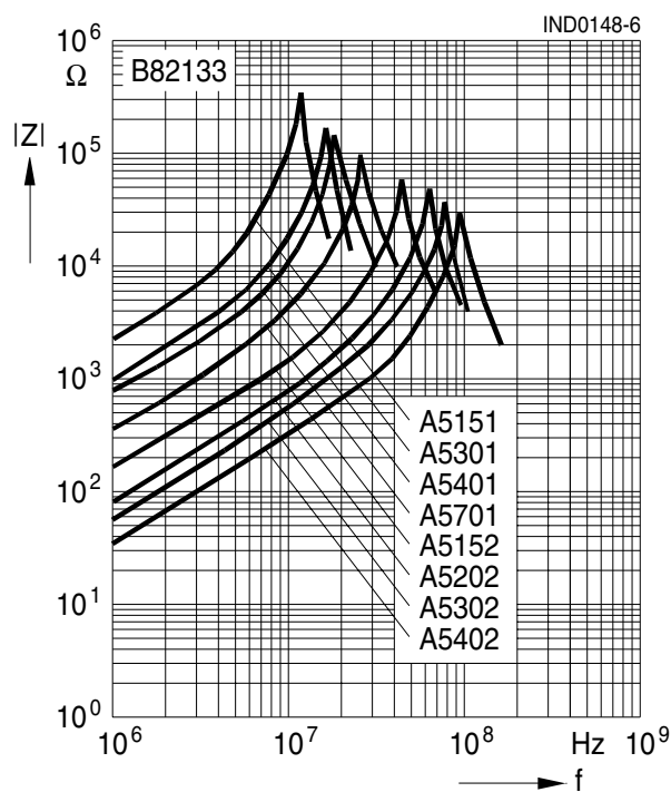
B82133A5***M000
