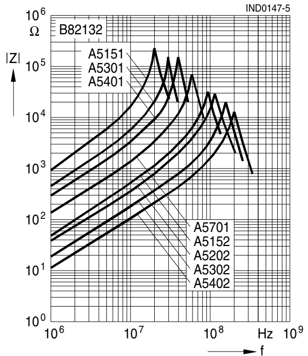
B82132A5***M000
